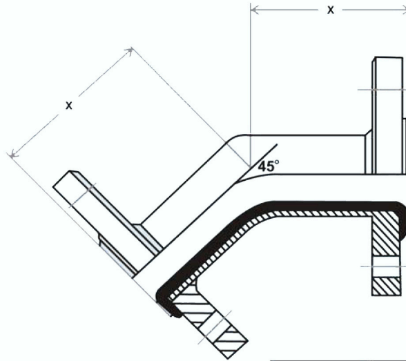
45 DEGREE ELBOW
